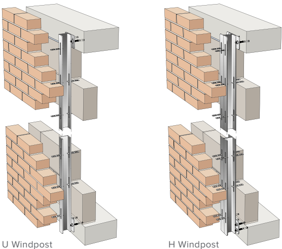
U Windpost
